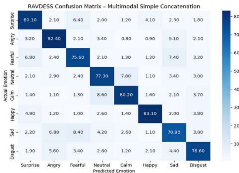
Figure 7. Confusion Matrix of multimodal simple concatenation on the RAVDESS Dataset
