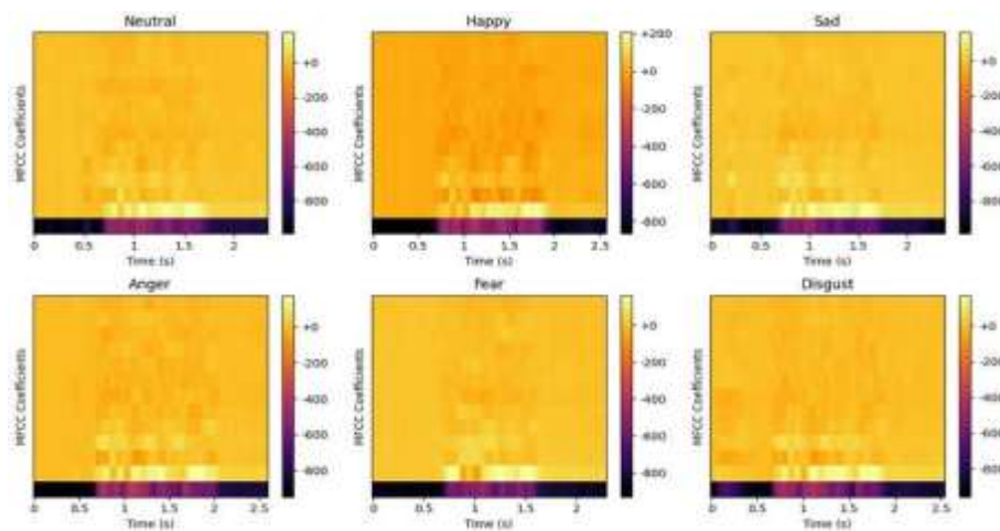
Figure 4. MFCC Spectrogram Extracted from RAVDESS Audio Sample for Emotion Classification.
